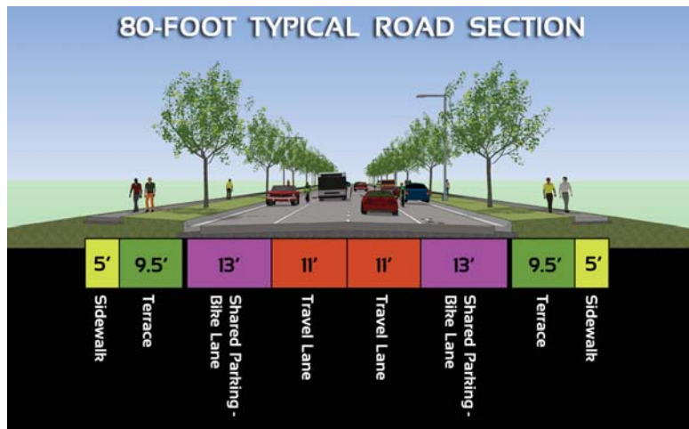
Figure 4.3: Typical Street Section, Avenue "A", Avenue "B", and Williamsburg Way
