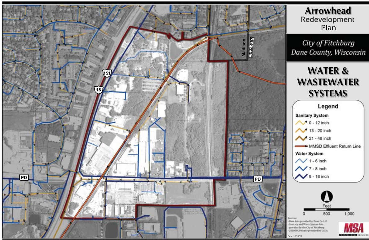
Figure 2.7: Water & Wastewater Systems
