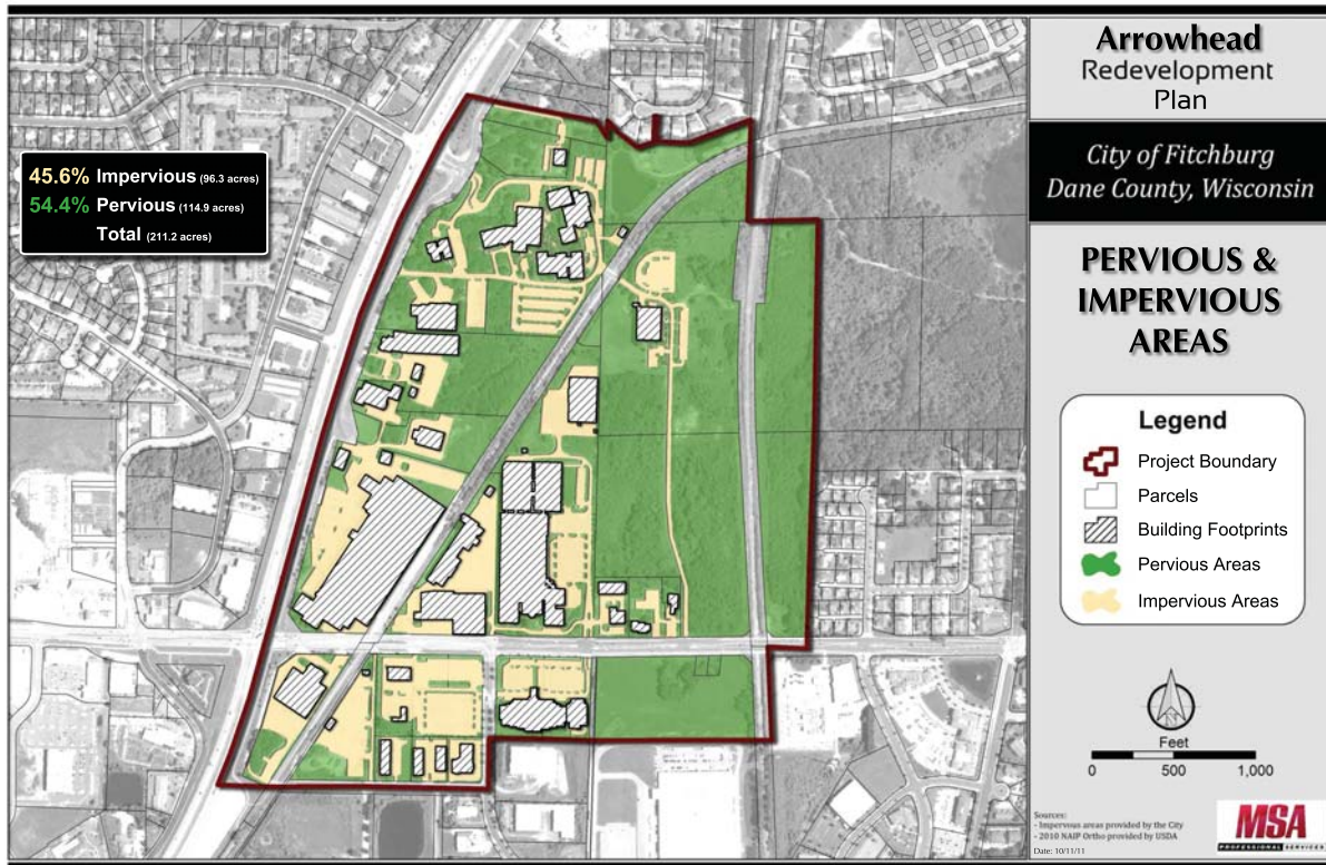
Figure 2.4: Pervious & Impervious Areas
