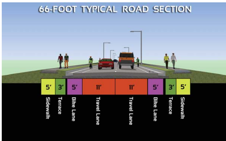
Figure 4.6: Typical Street Section, Cul-de-sac
