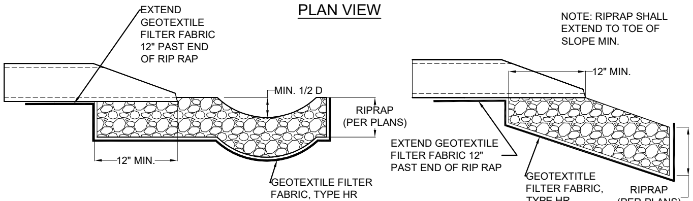
SLOPED/FLAT SWALE DISCHARGE AND FLAT POND DISCHARGE
