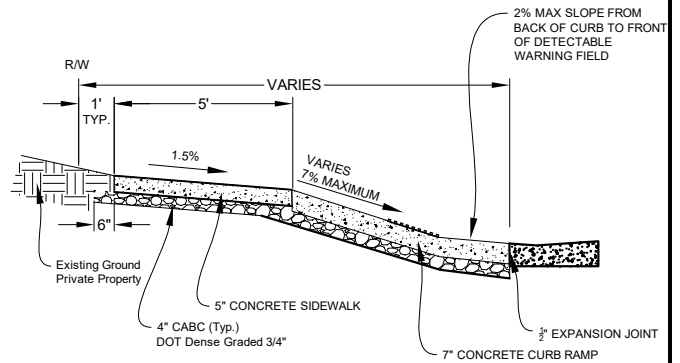
CURB RAMP TYPICAL SECTION
