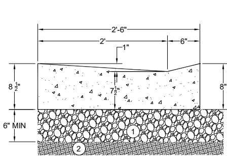
30" DRIVEWAY SECTION
