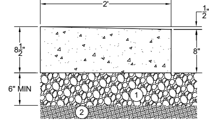
24" GUTTER
